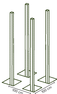
4 poteaux 9/9 JT008
